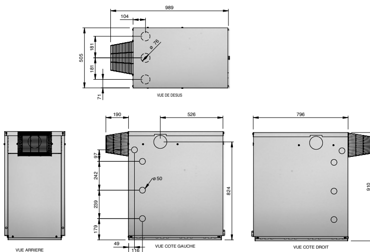
Dimensions chaudières Vortex Outdoor Bas NO x 32 kW
